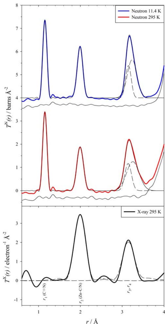
Figure 8. Peak fits to T^N(r) at 11.4 and 295 K (upper frame). The individual components (correlations r_3 and r_4 ) of the third peak are shown by dashed lines, and the residual is shown by a displaced continuous line (see parameters in Table 3 and Supporting Information Table S.13). For T^X(r) at 295 K (lower frame), the dashed lines indicate a partial fitting of r_2 , r_3 , and r_4 (see parameters in Supporting Information Table S.14).
